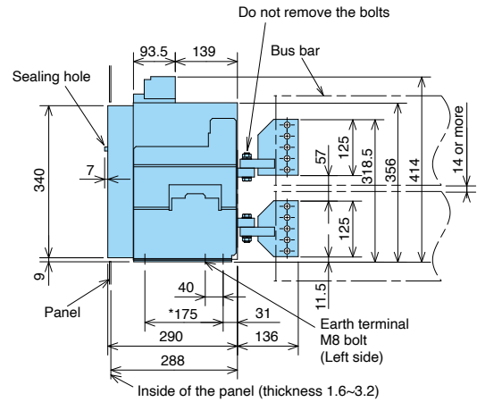
Main circuit terminal dimension
